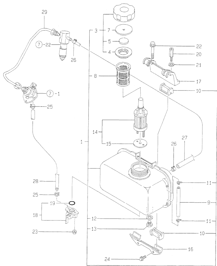
8.FUEL TANK & FUEL LINE
